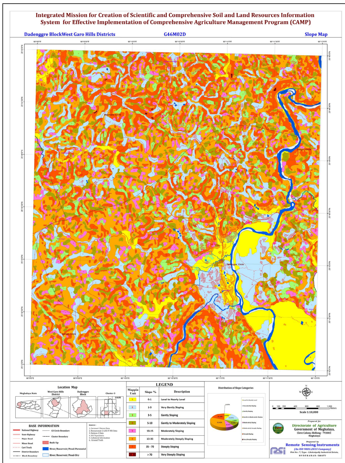
Figure-41: Slope Map of a Grid
