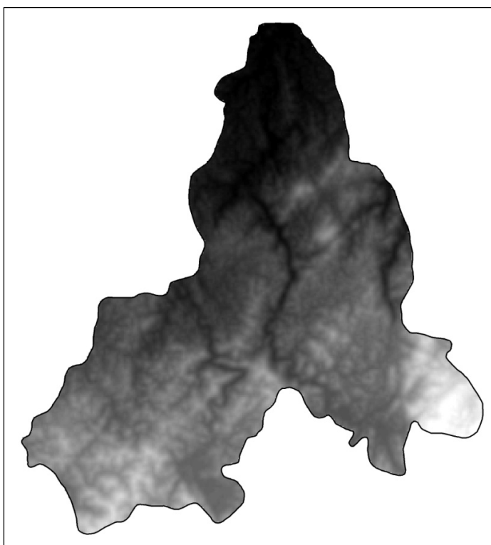
Figure-17: DEM Generated from Cartosat-1 Stereo Data
