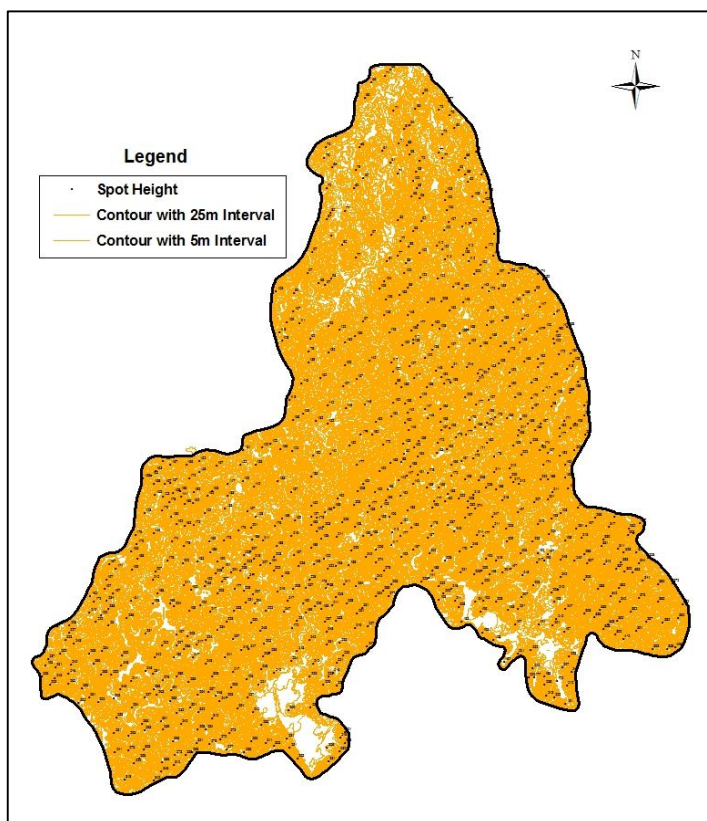
Figure-18: Part of Contours Generated from DEM
